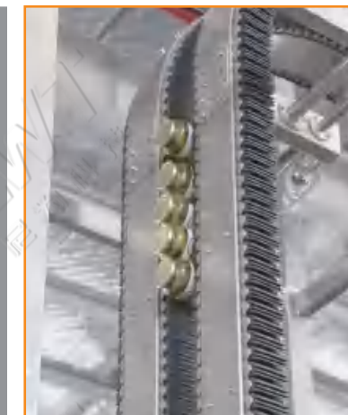
夹持垂直提升输送 Claping Type Vertical Lifting Conveyor
